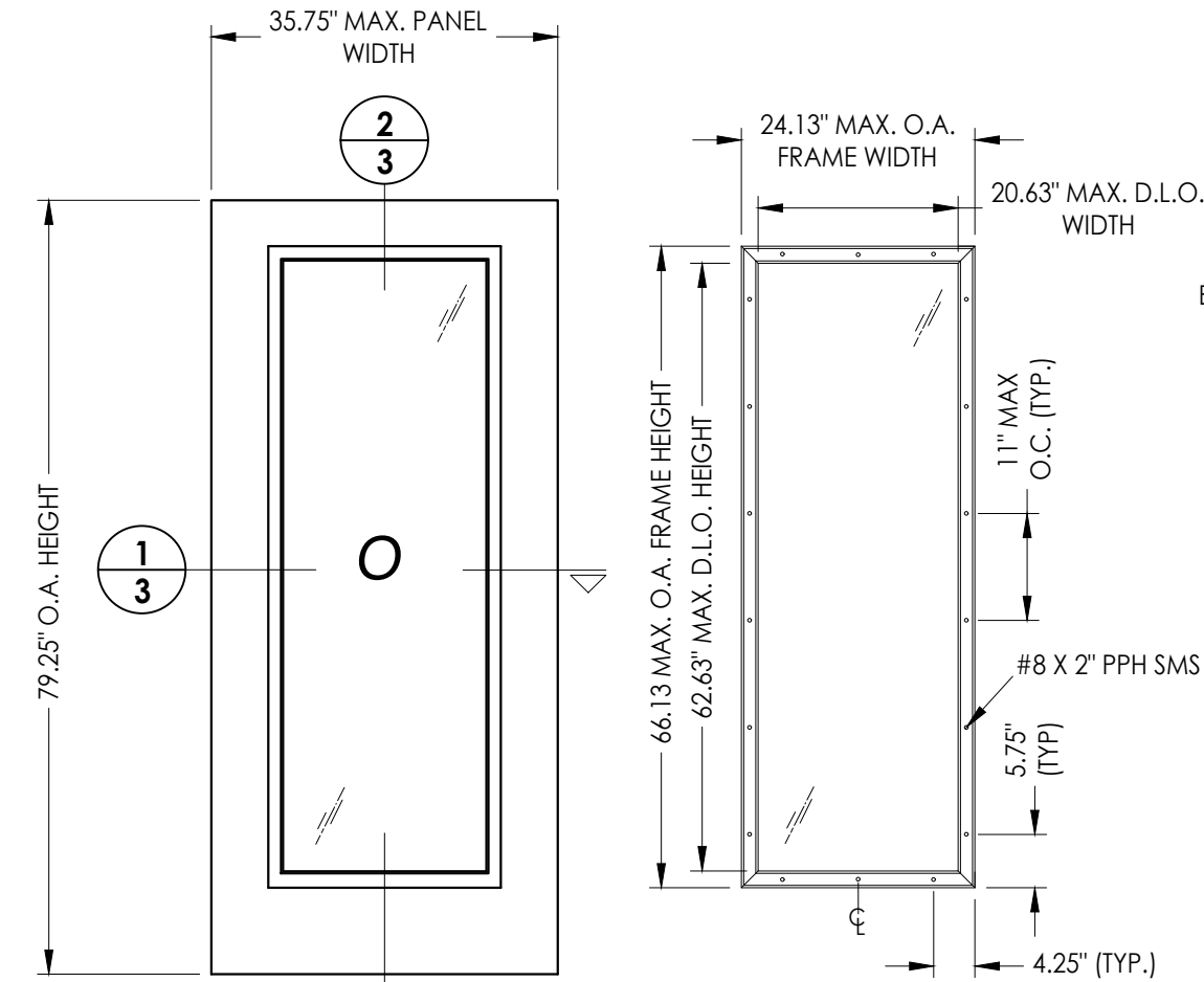
ODL LITE FRAME DETAIL "FLAT FRAME" PROFILE
